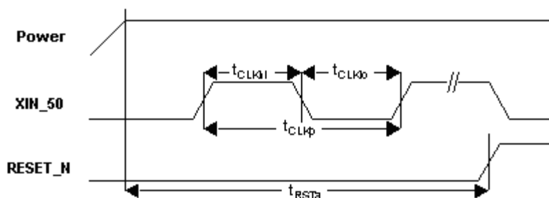
Figure 11: System Clock and Reset Timing
