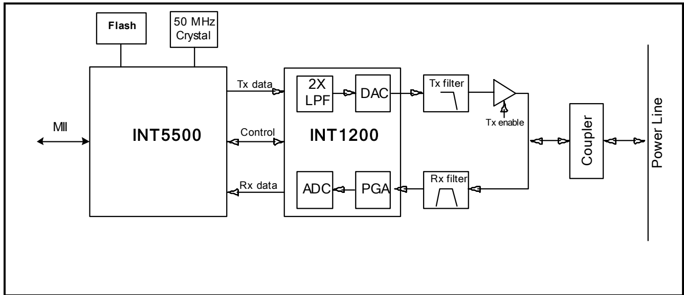
Figure 1: A General System Block Diagram of an INT5500CS based Powerline Device
