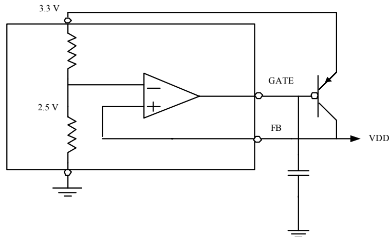
Figure 3. Voltage Regulator
