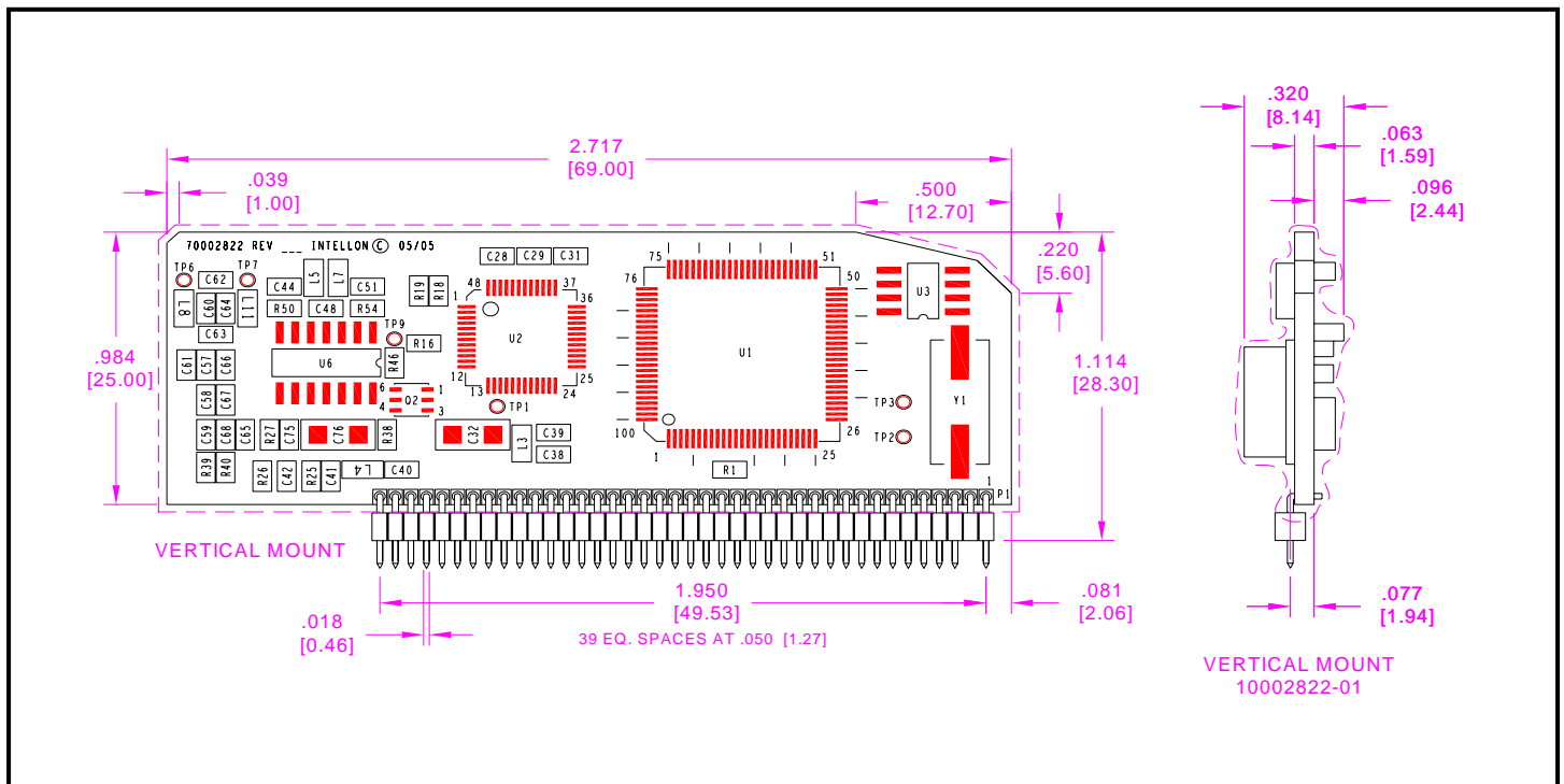
Figure 3: INT55MX Module with Right-Angle Connector
