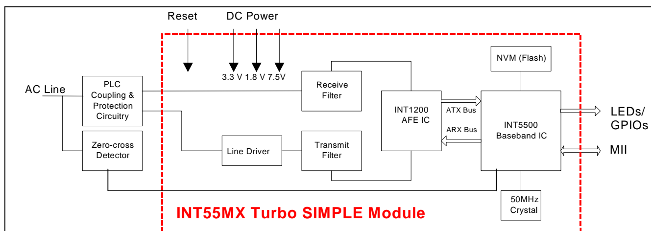
INT55MX Turbo SIMPLE Module Block Diagram
