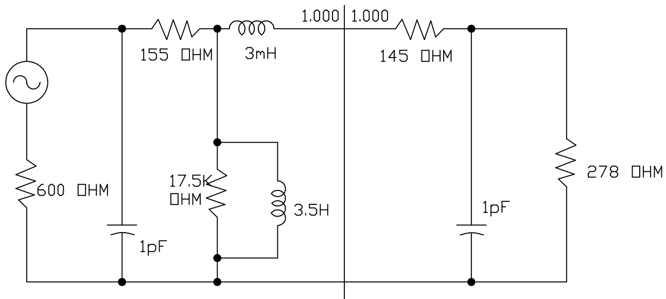
ATS-274X SPICE MODELING
