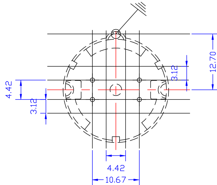
UNDERSIDE VIEW
