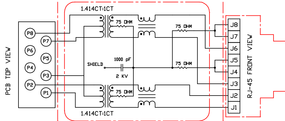
BLOCK CIRCUIT × 1 SET IN ATM-073E
