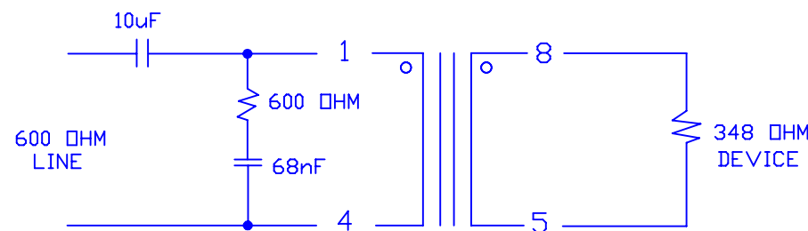
OPTIMUM CLASS (B) 600 Ω MATCH
