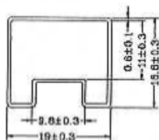
TUBE MECHANICAL DIMENSION
