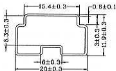
TUBE MECHANICAL DIMENSION
