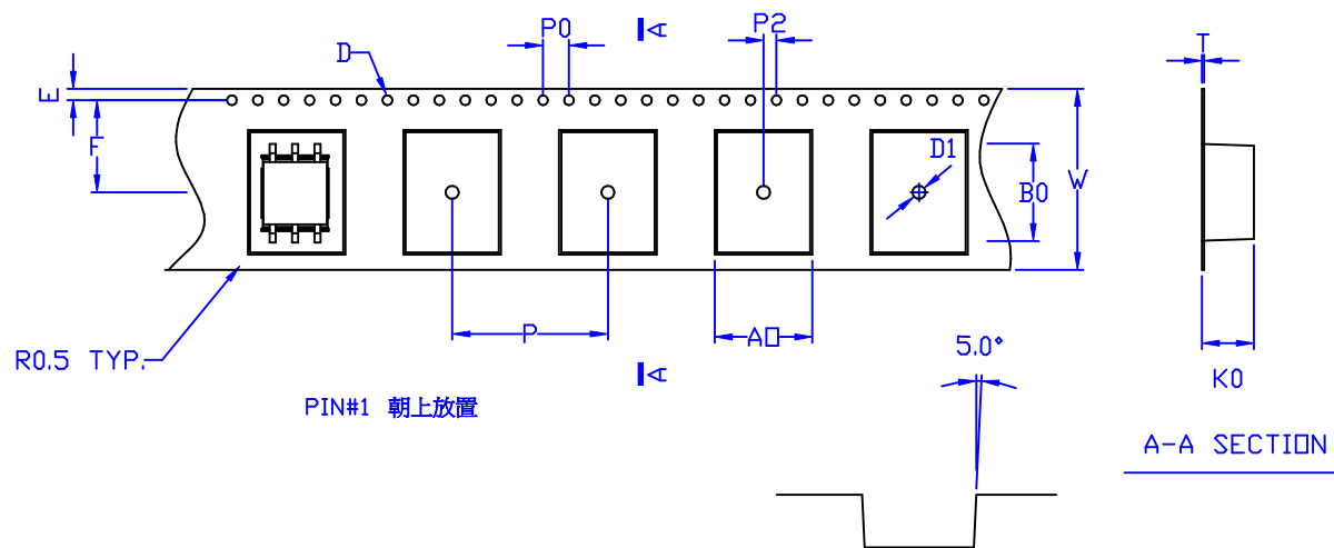
CARRIER TAPE
