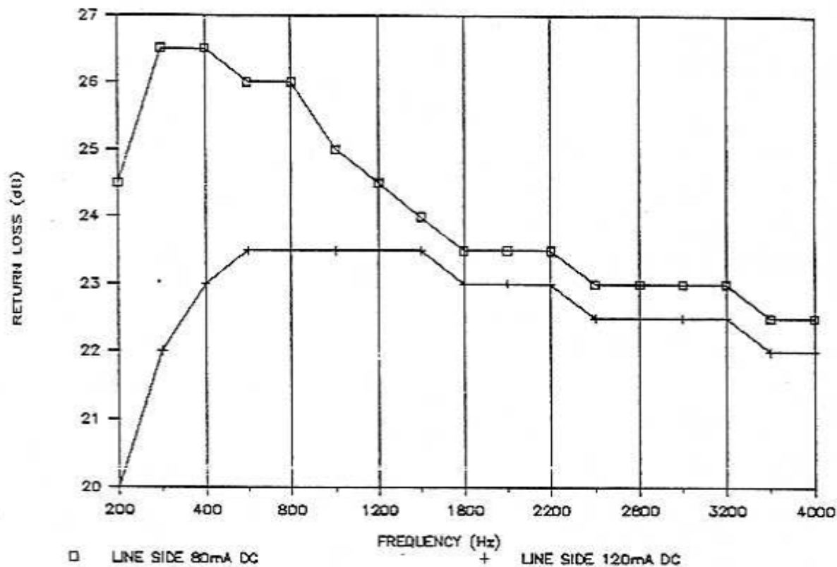
Return Loss vs Frequency
