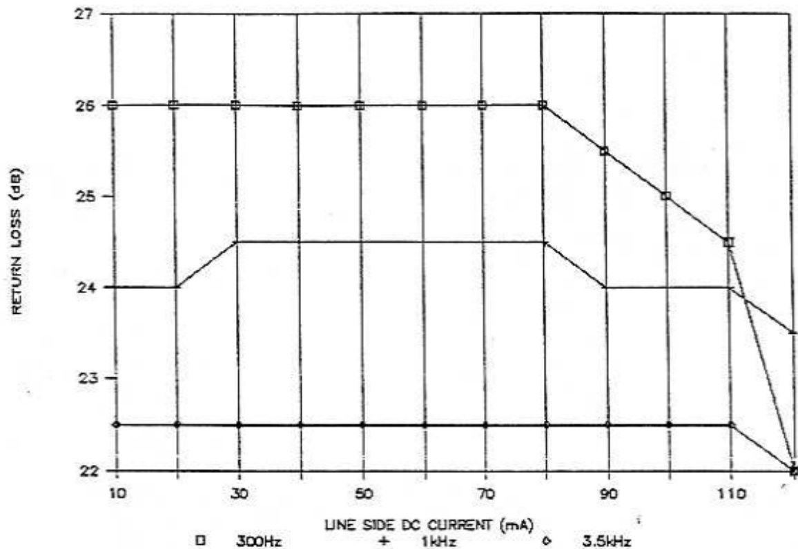
Return Loss vs Line Side DC Current
