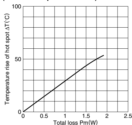
Temperature rise vs. Total loss for ETD24 core (Typical) (Ambient temperature: 25°C)
