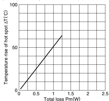
Temperature rise vs. Total loss for SEE16 core (Typical) (Ambient temperature: 25°C)
