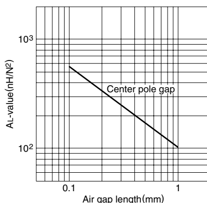
AL-value vs. Air gap length for PC40ETD24 core (Typical)
