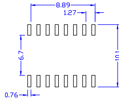
RECOMMENDED PAD LAYOUT
